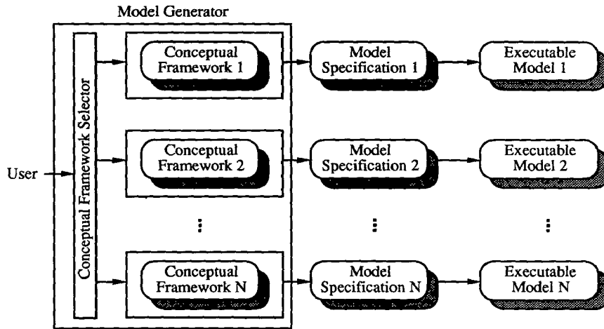
Figure 3. Model Generator Construction Approach 2
