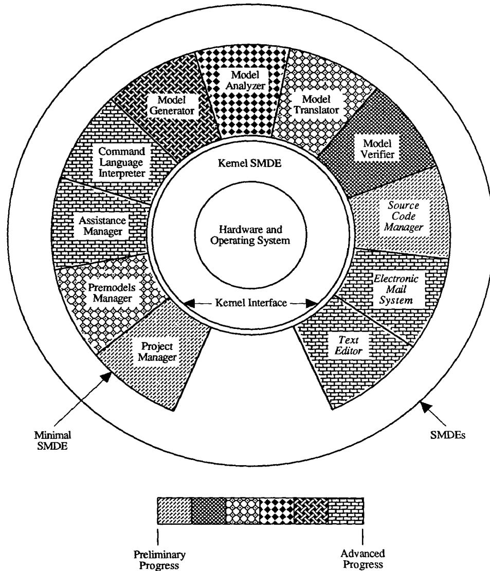
Figure 1. The Architecture of the SMDE and Current Status of Each Minimal SMDE Tool
